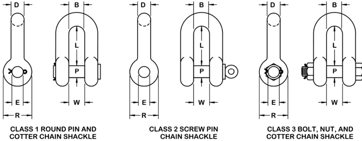
FIGURE 20. Type IV, grade B, chain shackles.
